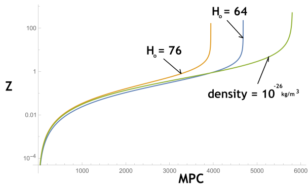
Figure 1 The trace labeled H_o were computed using equation 11. 1 MPC = 3.262 \times 10^6 light years = 3.086 \times 10^{22} meters for an expanding universe. Below 3 MPC Hubble calculated response varies little. The other curve was computed from equation 10 for photon propagation. What is interesting is the Hubble result almost matches the gravitational red shift over lower Z values where the mean density of the universe is 10^{-26} \text{ kg/m}^3 .
